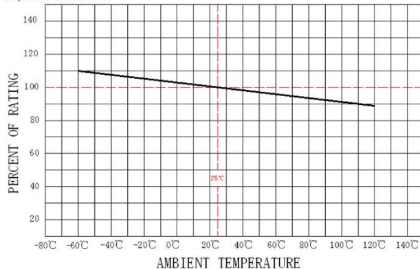
Temperature-Current curve:
