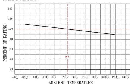
Temperature-Current curve:
